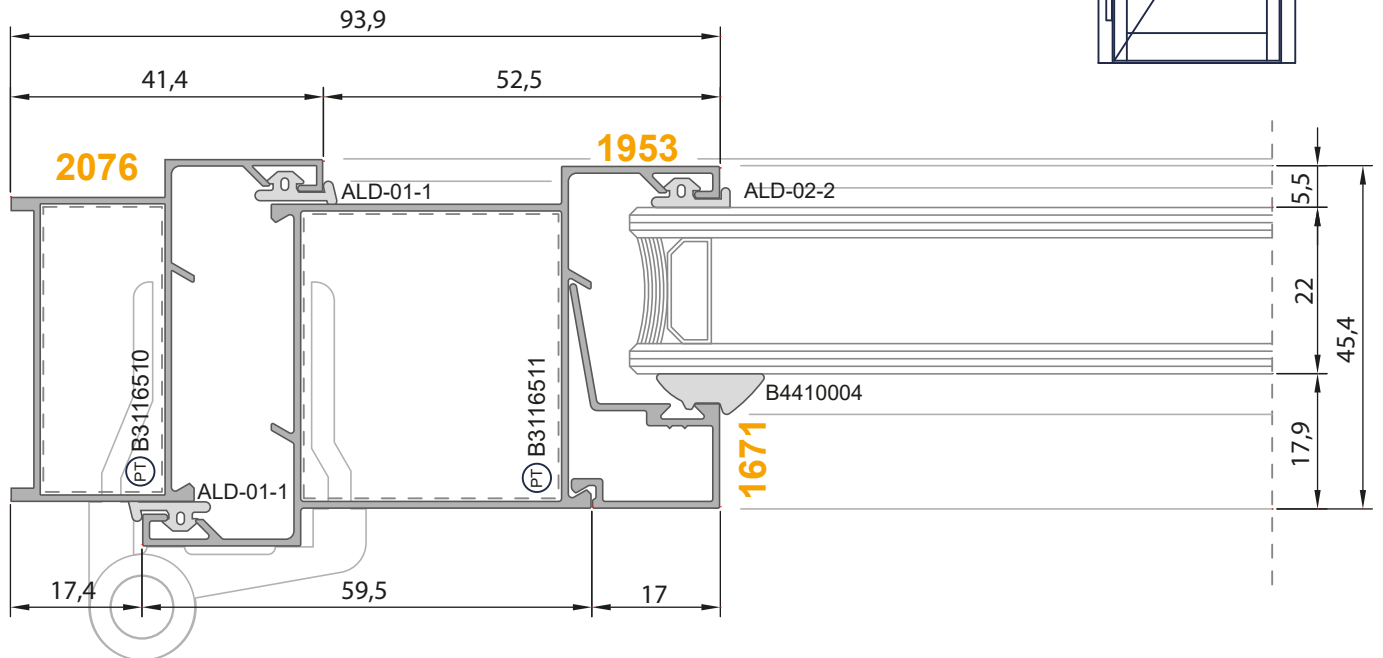
14-14 Detay
