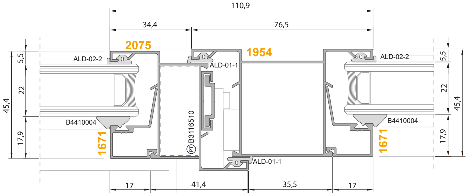
12-12 Detay
