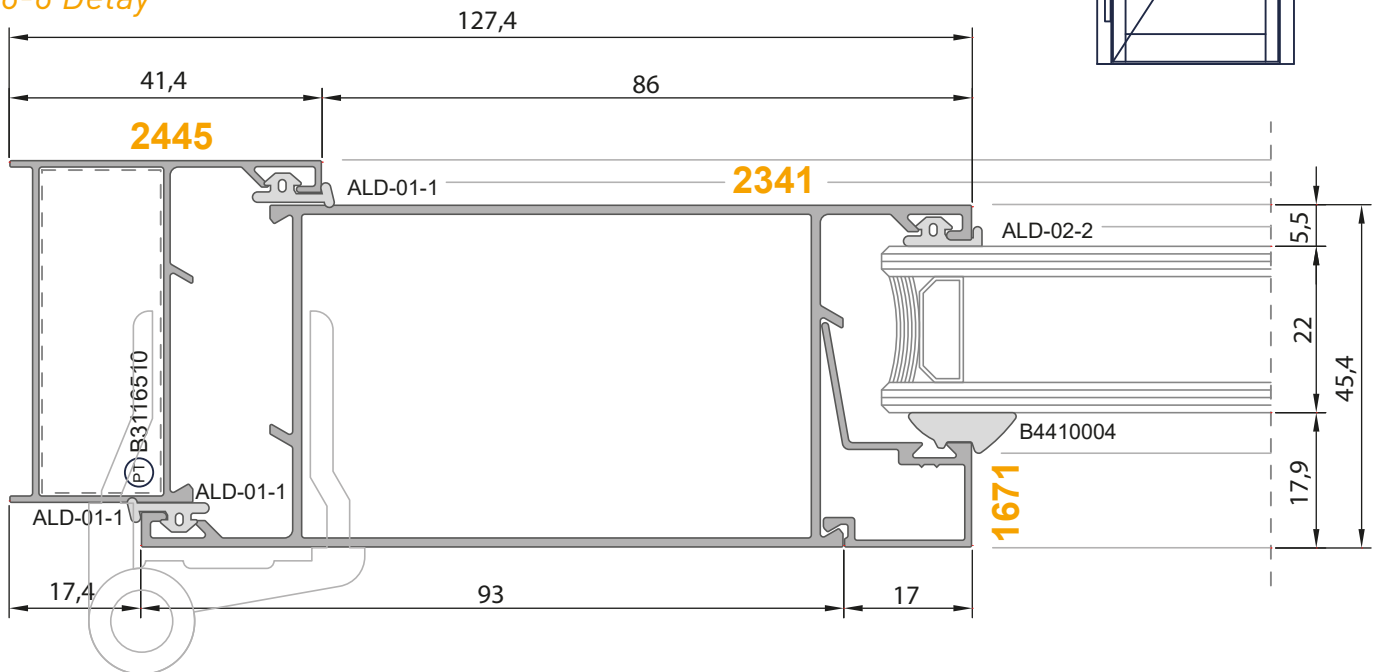
6-6 Detay
