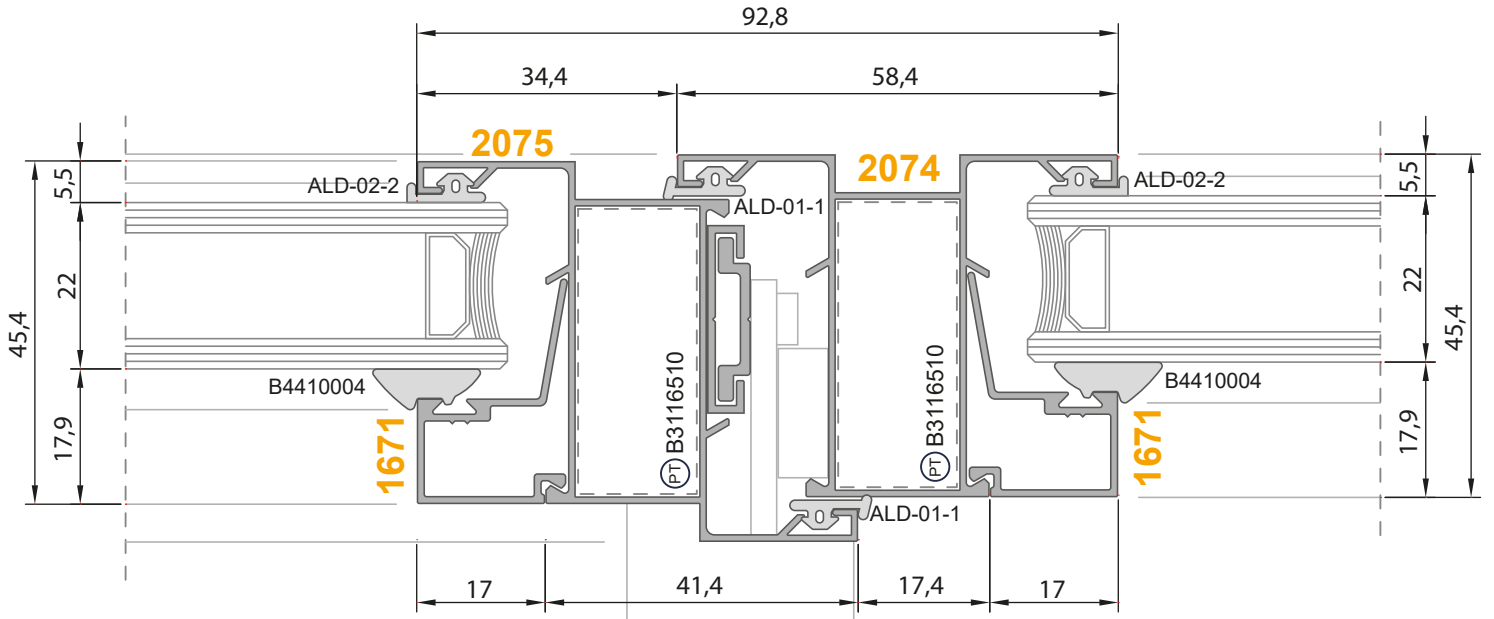
12-12 Detay
