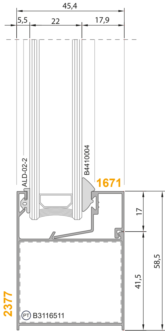
1-1 Detay
