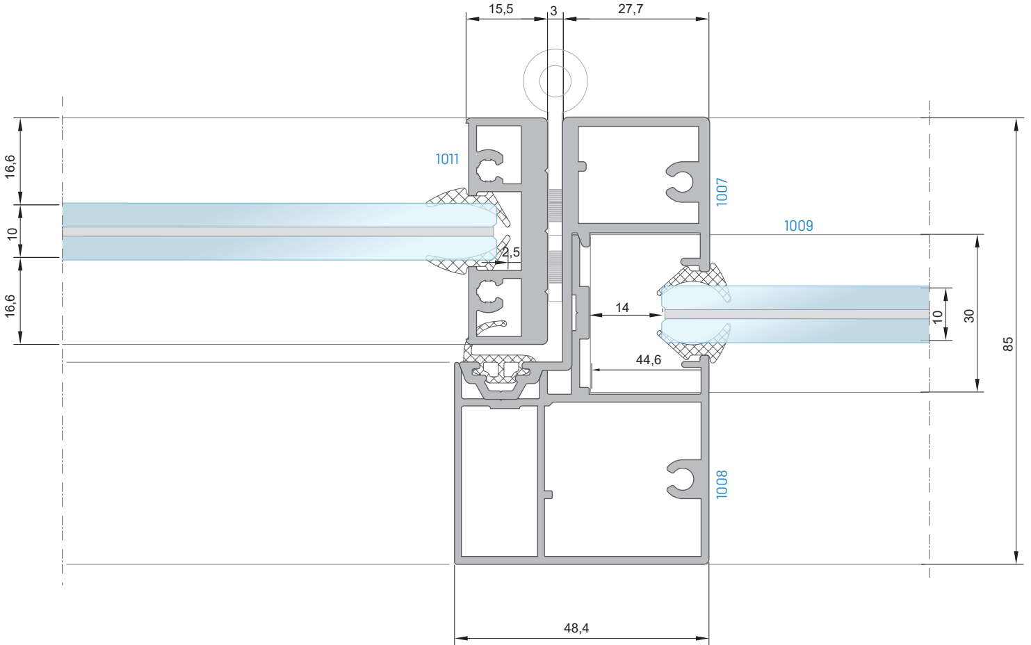
14:14 DETAY 14:14 DETAIL
