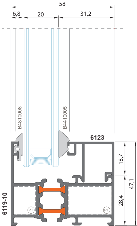
Detay 1 Detail 1
