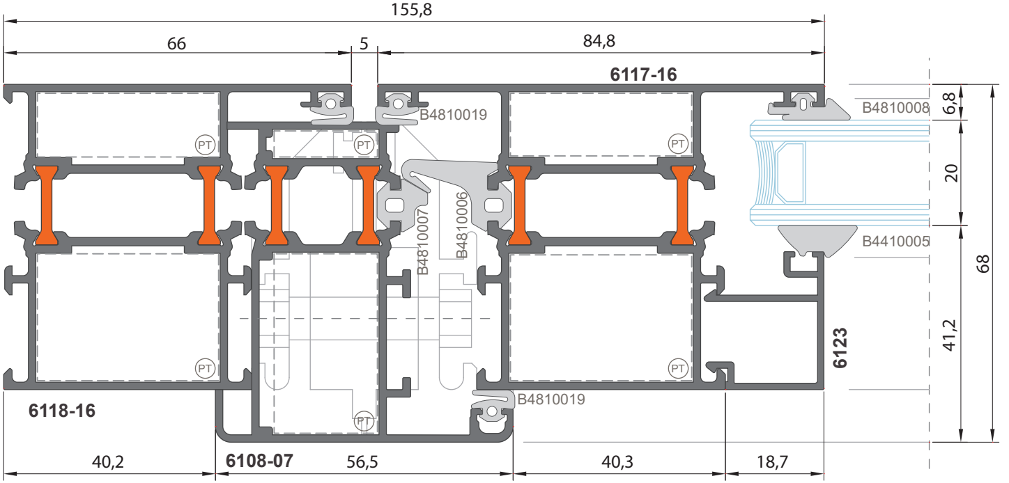
Detay 8 Detail 8
