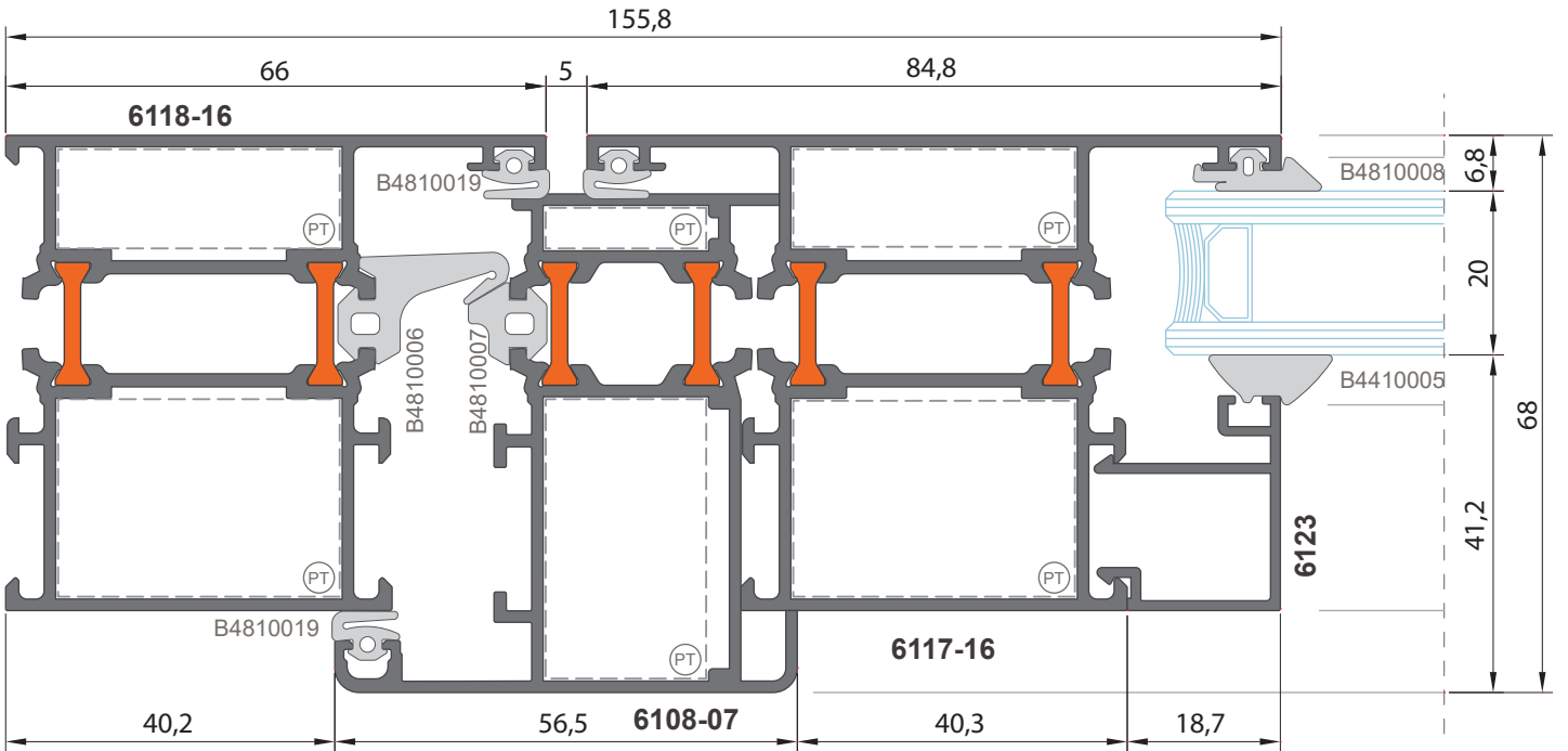
Detay 9 Detail 9
