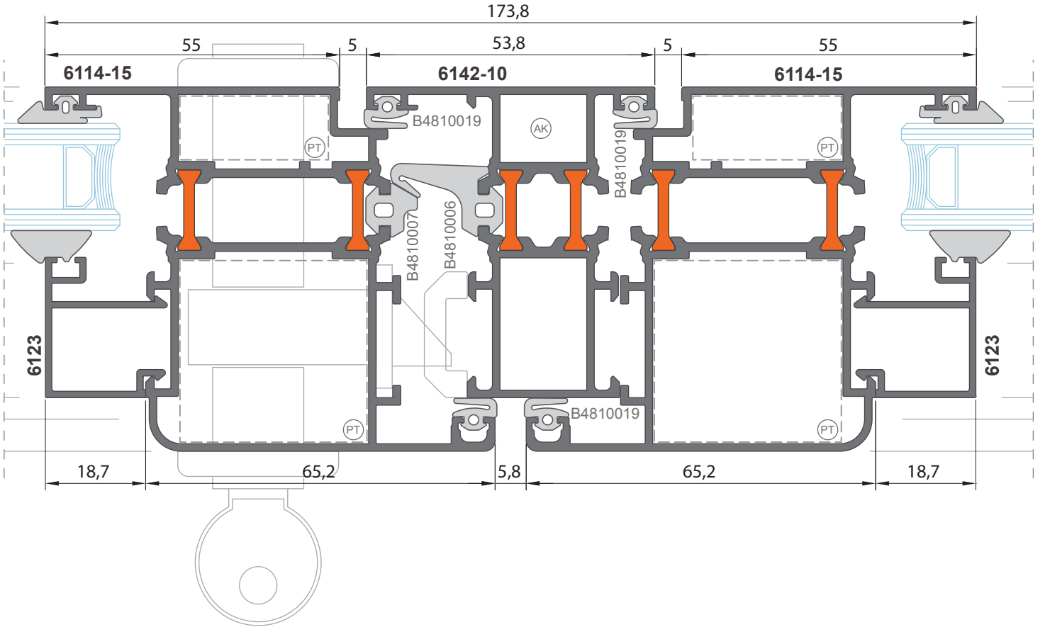
Detay 18 Detail 18
