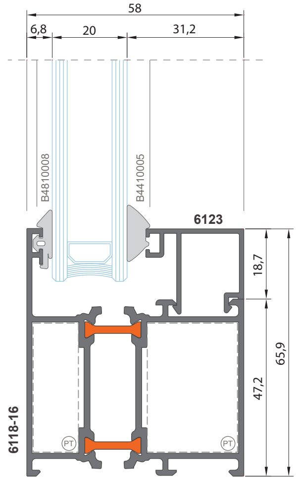
Detay 1 Detail 1
