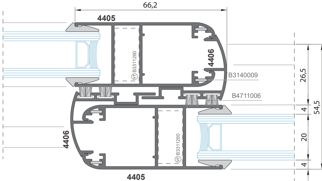
3-3 Detay 3-3 Detail
