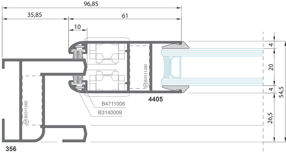
2-2 Detay 2-2 Detail
