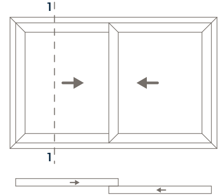
1-1 Detay 1-1 Detail
