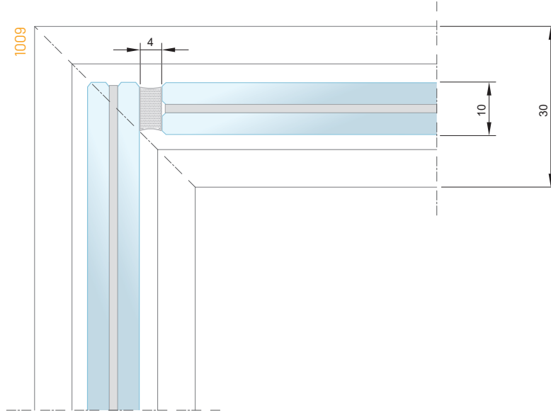
6:6 DETAY 6:6 DETAIL
