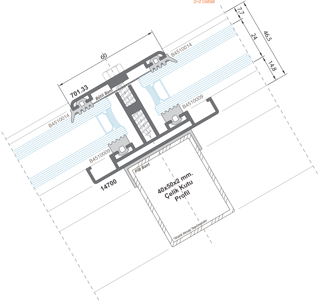
2-2 Detay 2-2 Detail
