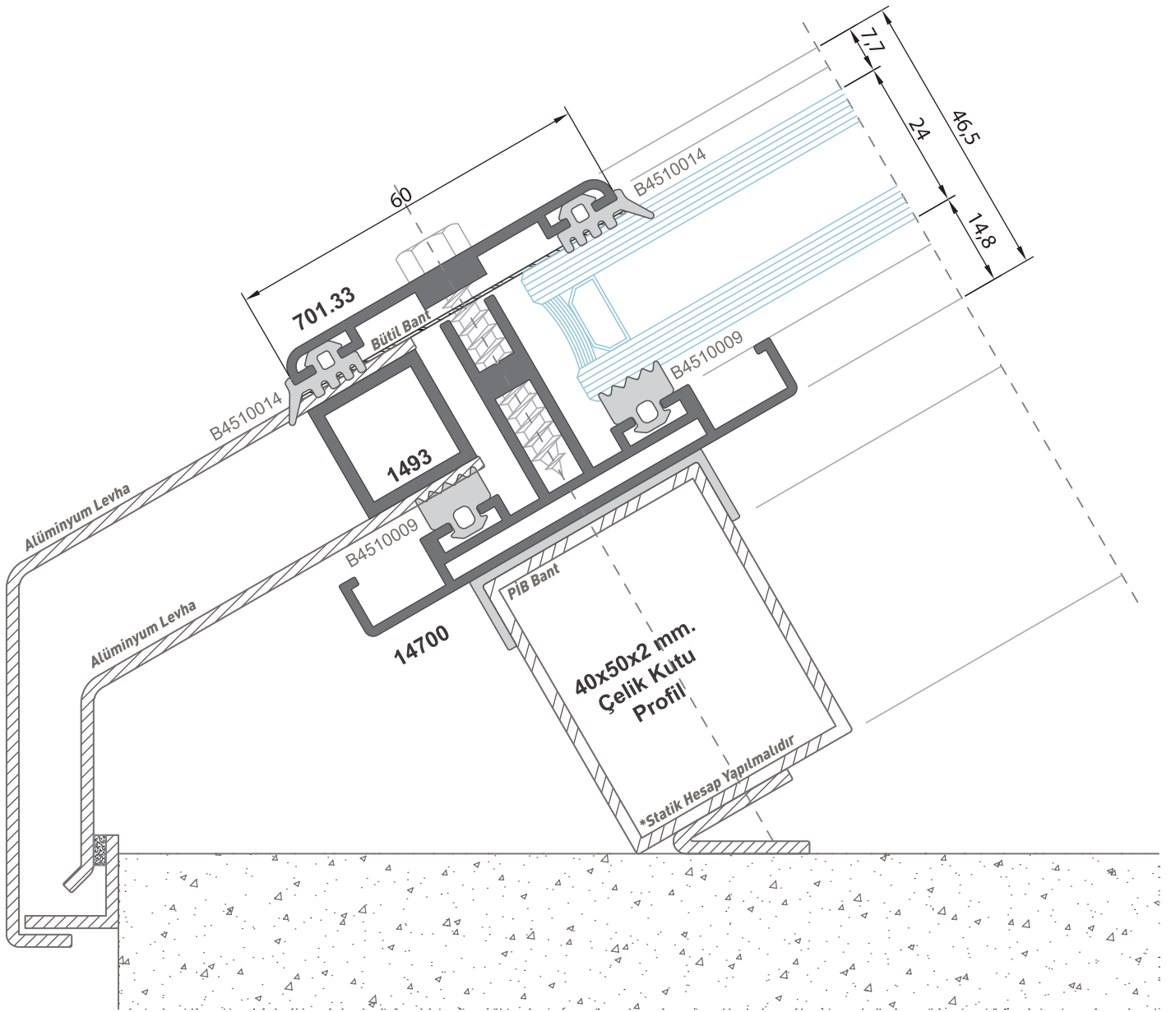
5-5 Detay 5-5 Detail
