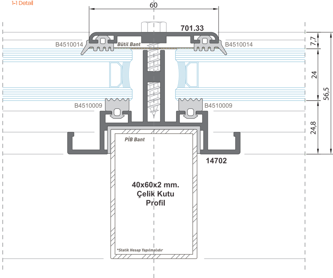
1-1 Detay 1-1 Detail
