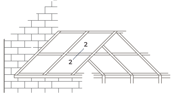
2-2 Detay 2-2 Detail
